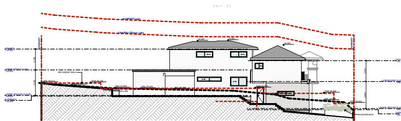
SOUTH ELEVATION UNIT 2 SCALE 1:500
