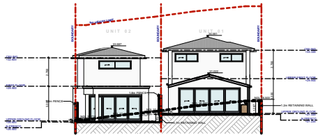
WEST ELEVATION SCALE 1:500
