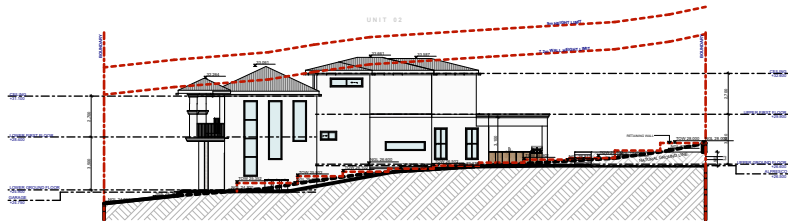
NORTH ELEVATION UNIT 2 SCALE 1:500
