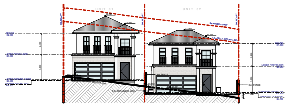
EAST ELEVATION SCALE 1:500
