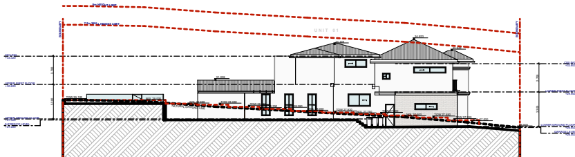
SOUTH ELEVATION UNIT 1 SCALE 1:500
